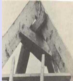
FIG. 5 LAYOUT SHOWS BASE CORNERS MITERED AT 45°. SIDE MEMBERS MITERED AT 38° FOR FITTING TO BASE, AND MITERED AT 52° FOR APEX.
