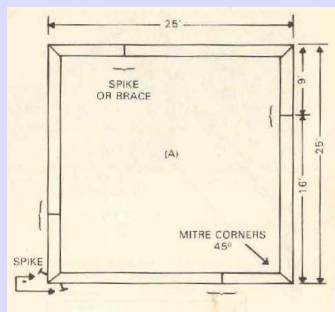
FIG. 5 LAYOUT SHOWS BASE CORNERS MITERED AT 45°. SIDE MEMBERS MITERED AT 38° FOR FITTING TO BASE, AND MITERED AT 52° FOR APEX.
