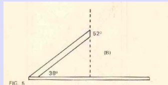
FIG. 5 LAYOUT SHOWS BASE CORNERS MITERED AT 45°. SIDE MEMBERS MITERED AT 38° FOR FITTING TO BASE, AND MITERED AT 52° FOR APEX.
